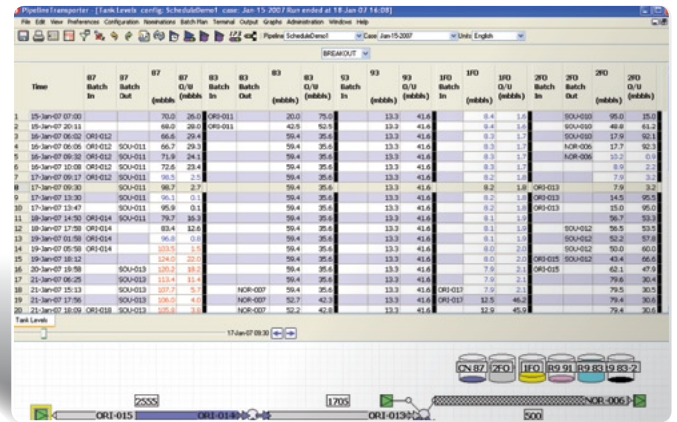
Simulation screens to track liquid scheduling
