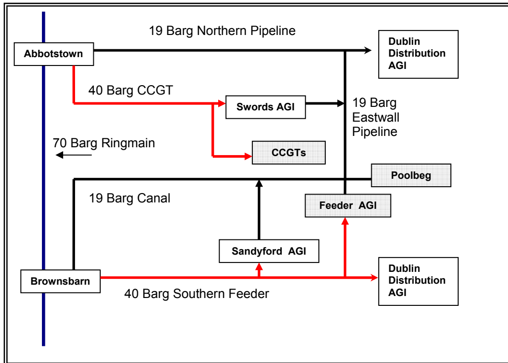
Figure 2: Dublin Transmission System Main Components
