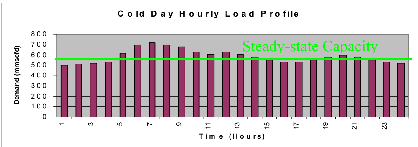
Chart 1: Chart illustrating how a load may change at a demand on a cold day
